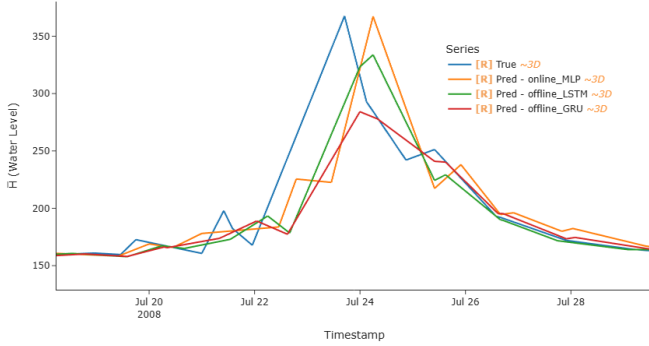
(b) Performance of Offline LSTM and GRU vs Online MLP.
